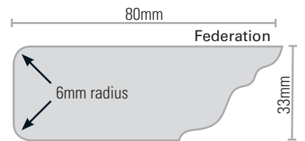
CAPPING MOULD
